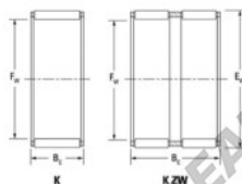
Boundary dimensions
