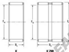
Rolls (needle roller and cage assemblies)
