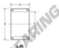
Boundary dimensions
