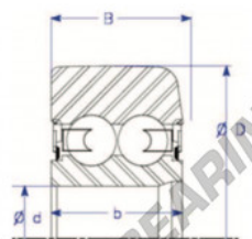
X-e: compact one-piece design Style X-e Double Row Ball Bearing
