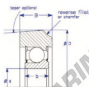
B Max-Type Style VII : Chamfer of reverse Fillet
